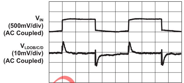
LDOB/C/D Line Transient
