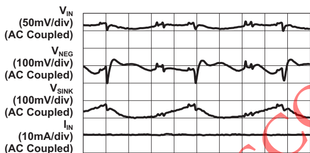
Backlight Operating Characteristics, 1.5X Mode (V_{IN} = 3.6V; I_{BLX} = 19.8mA/ch)
