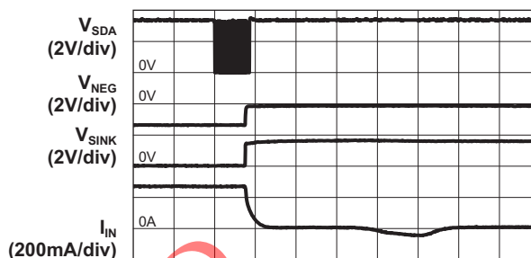
Backlight Turn OFF Characteristics, 1.5x Mode (V_{IN} = 3.6V; I_{BLX} = 19.8mA/ch)
