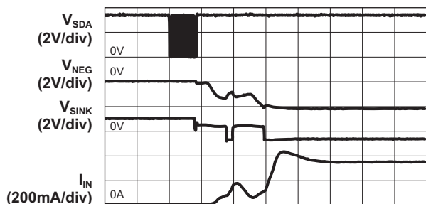
Backlight Turn ON Characteristics, 2x Mode (V_{IN} = 3.0V; I_{BLX} = 19.8mA/ch)
